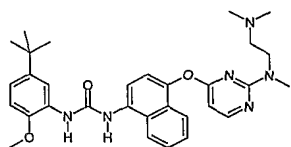
1-(5-tert-Butyl-2-methoxy-phenyl)-3-(4-{2-[(2-dimethylamino-ethyl)-methyl-amino]-pyrimidin-4-yloxy}-naphthalen-1-yl)-urea;
